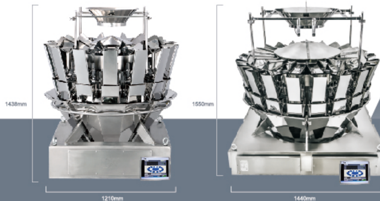
AC-6B14-4A -24 (14 Heads)
