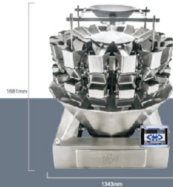
AC-6B14-4A-21 (14 heads)
